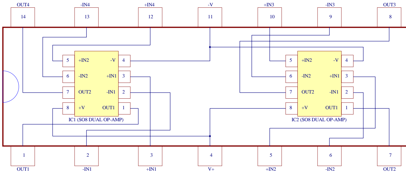
QUAD OP-AMP DIP PACKAGE (STANDARD QUAD PINOUT)
