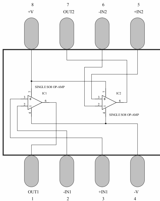
SINGLE TO DUAL OP-AMP / SO8 TO SO8
