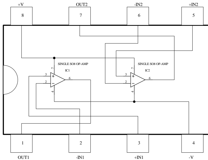
DUAL OP-AMP DIP PACKAGE
